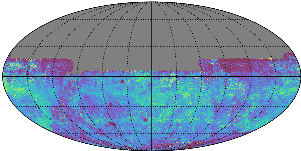
extra_ss_neo2_v3.4_10yrs All sky y band: 75th Percentile Intranight Timespan
