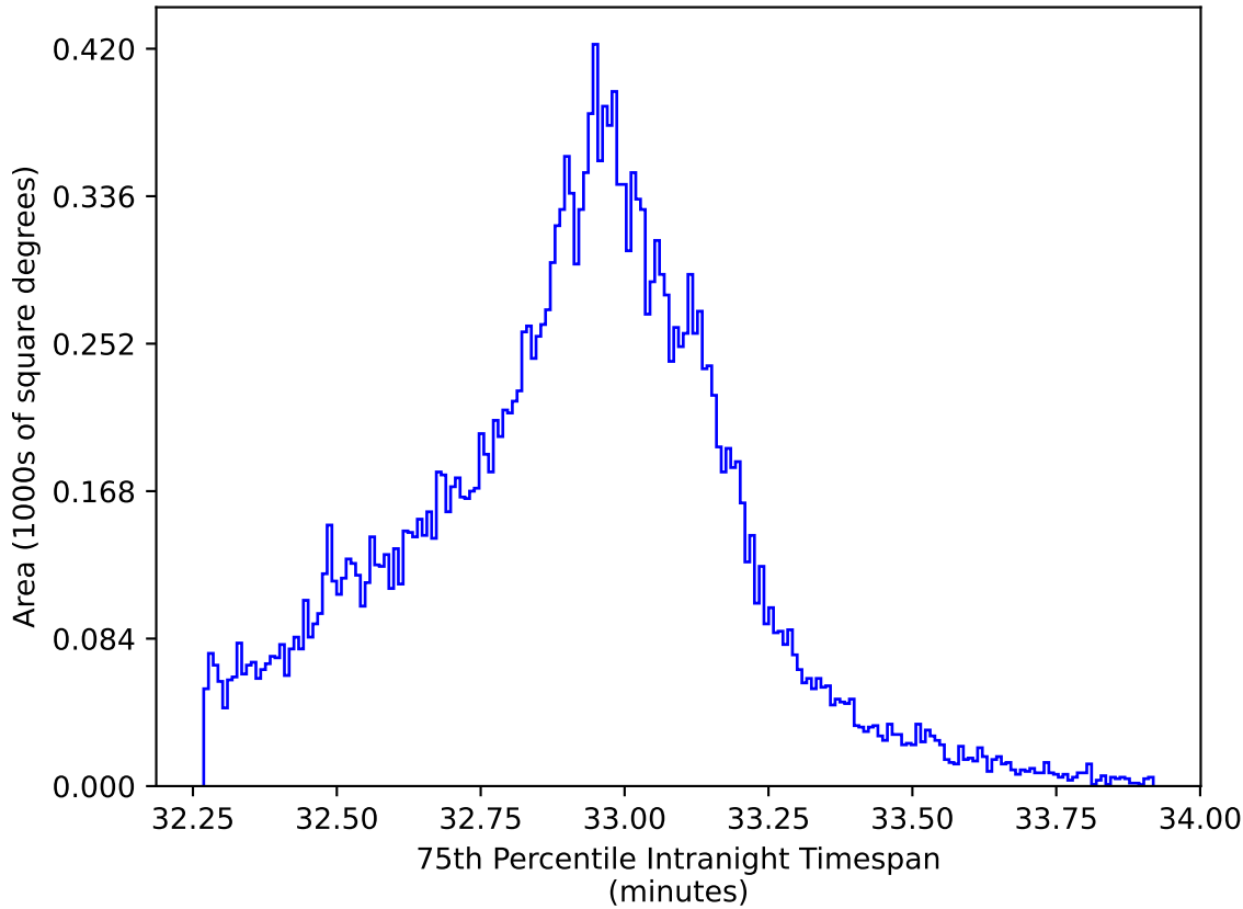
extra_ss_neo2_v3.4_10yrs All sky y band: 75th Percentile Intranight Timespan
