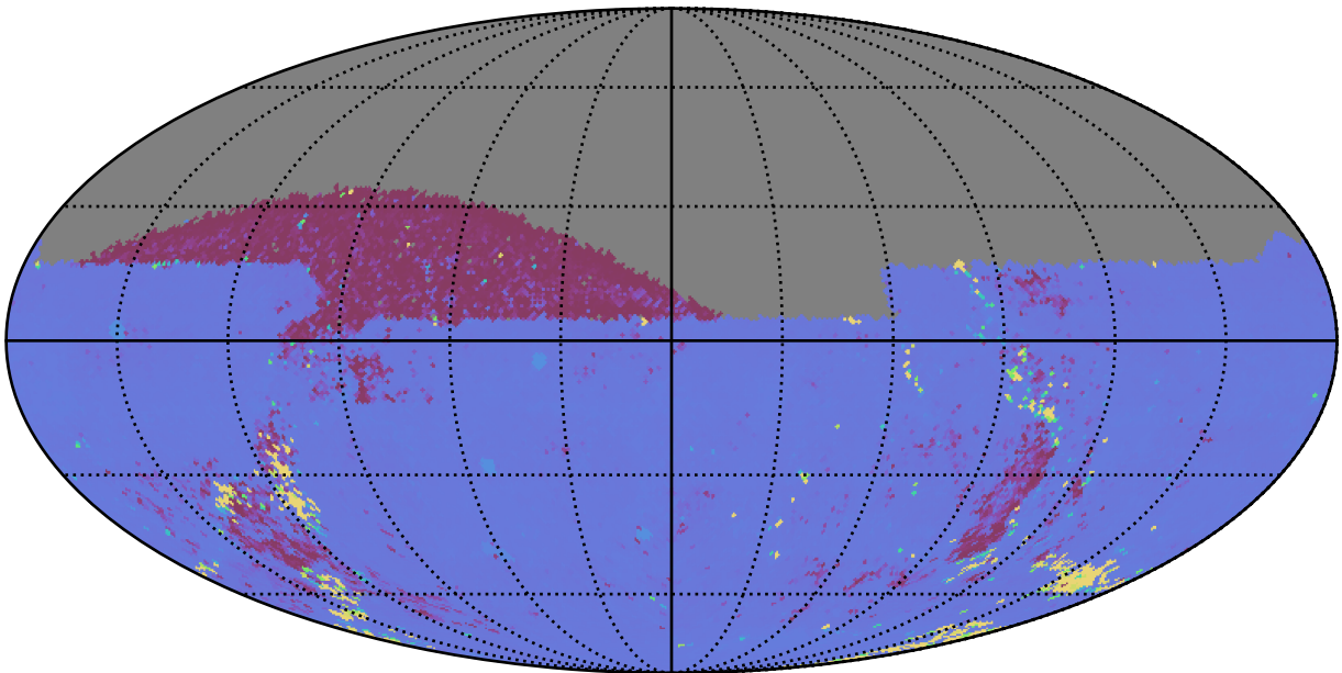
extra_ss_neo2_v3.4_10yrs All sky ug bands: 75th Percentile Intranight Timespan
