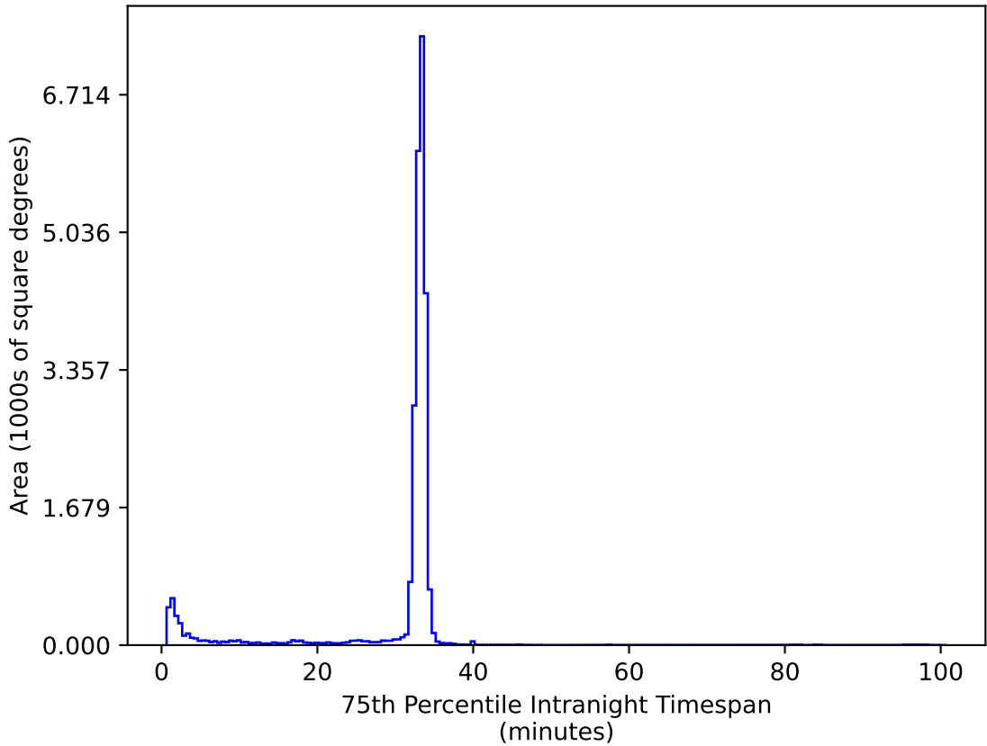
extra_ss_neo2_v3.4_10yrs All sky ug bands: 75th Percentile Intranight Timespan
