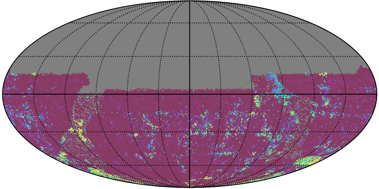
extra_ss_neo2_v3.4_10yrs All sky u band: 75th Percentile Intranight Timespan
