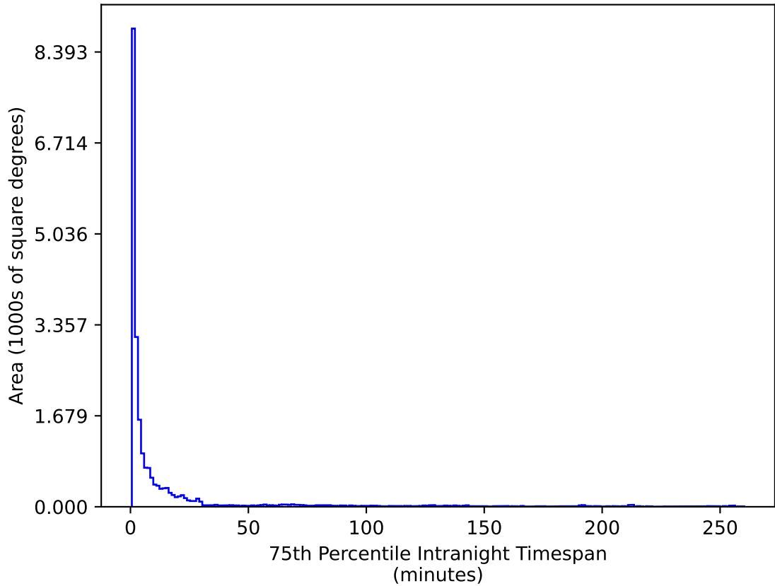
extra_ss_neo2_v3.4_10yrs All sky u band: 75th Percentile Intranight Timespan
