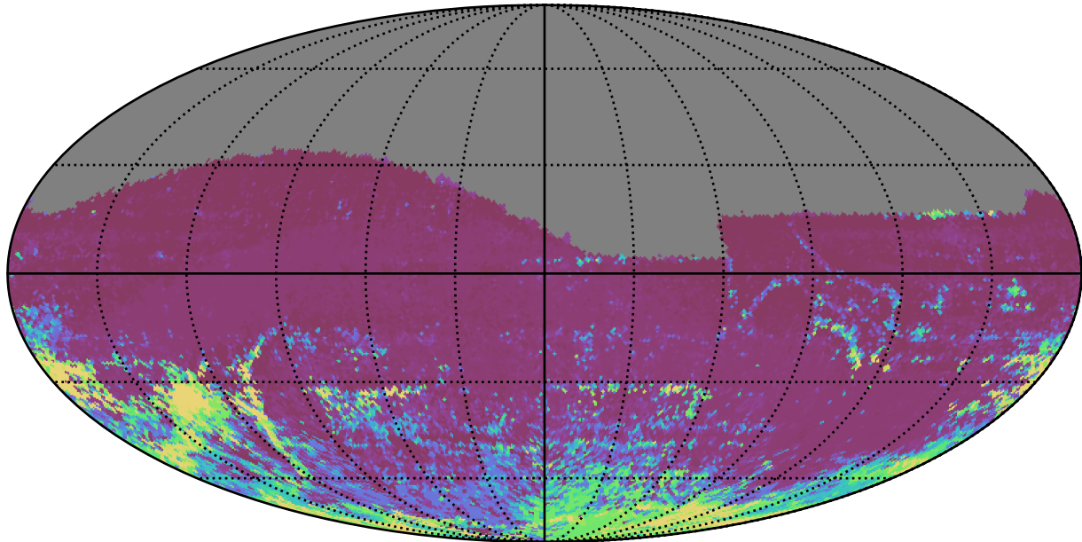
extra_ss_neo2_v3.4_10yrs All sky r band: 75th Percentile Intranight Timespan
