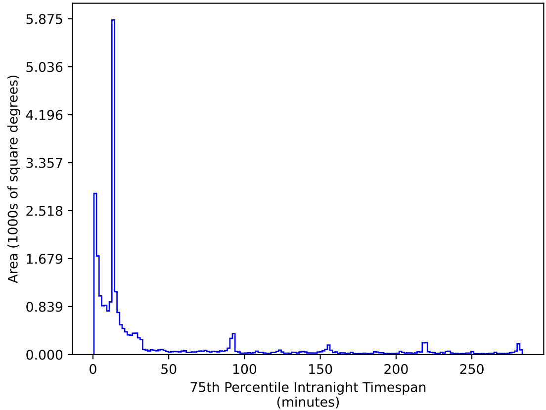
extra_ss_neo2_v3.4_10yrs All sky r band: 75th Percentile Intranight Timespan
