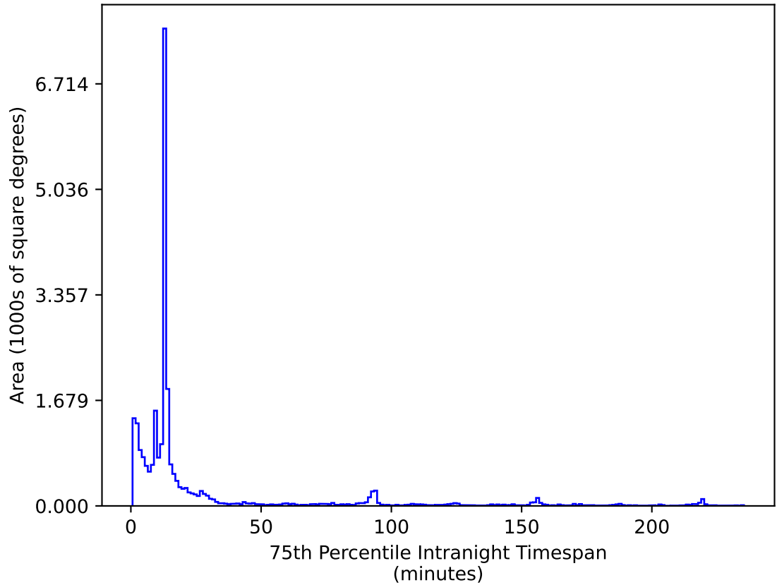
extra_ss_neo2_v3.4_10yrs All sky i band: 75th Percentile Intranight Timespan
