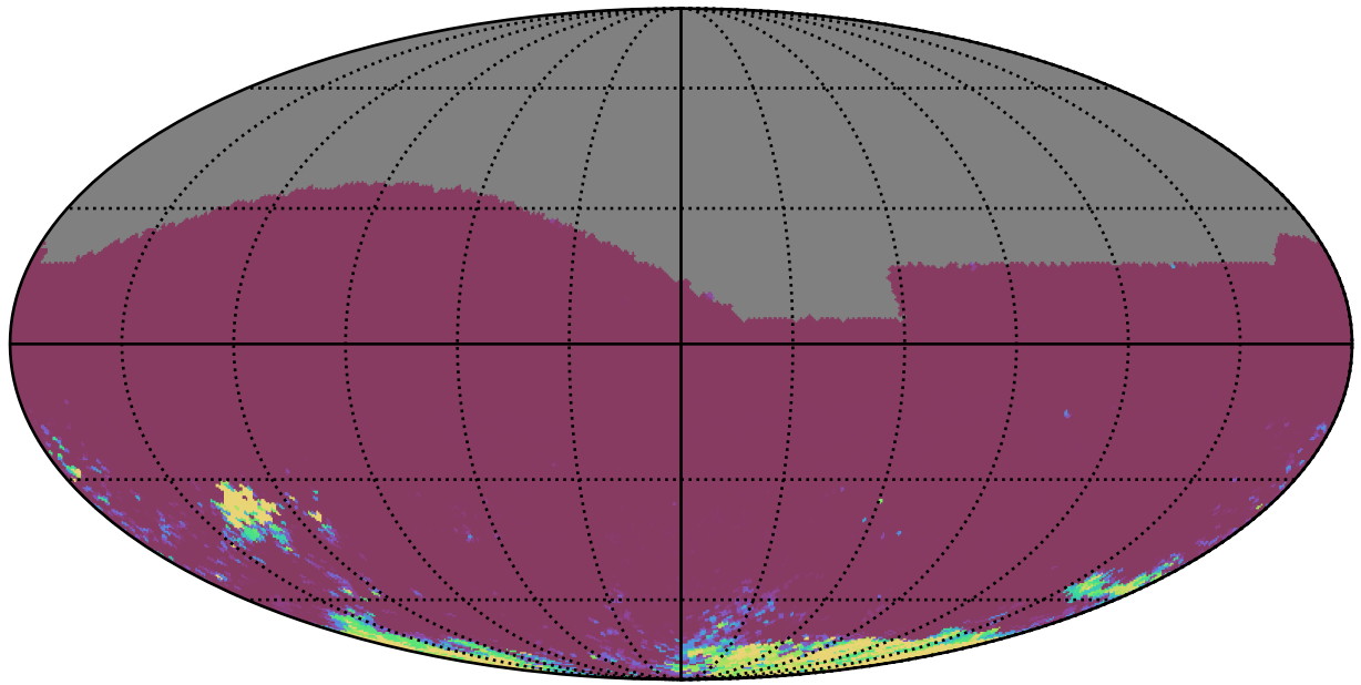
extra_ss_neo2_v3.4_10yrs All sky gr bands: 75th Percentile Intranight Timespan
