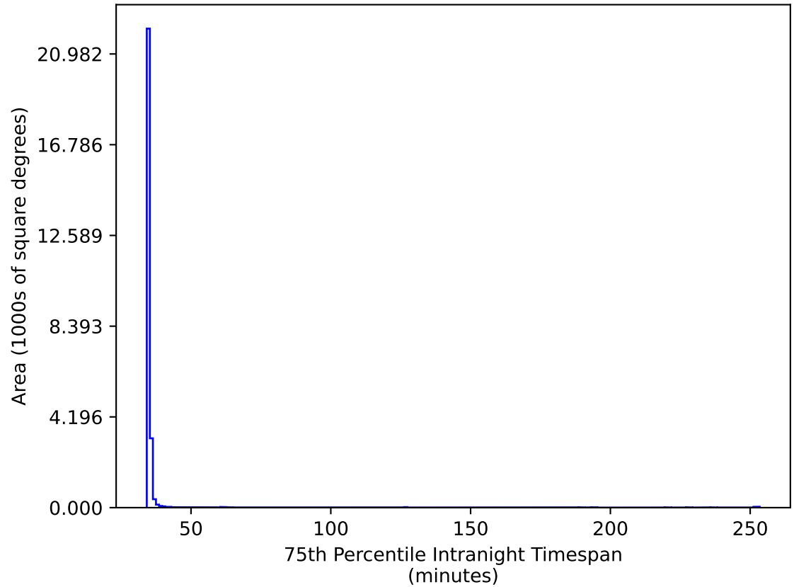
extra_ss_neo2_v3.4_10yrs All sky gr bands: 75th Percentile Intranight Timespan
