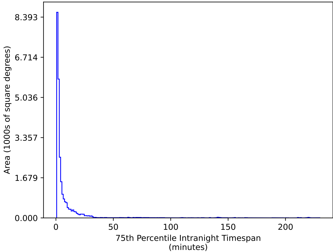
extra_ss_neo2_v3.4_10yrs All sky g band: 75th Percentile Intranight Timespan
