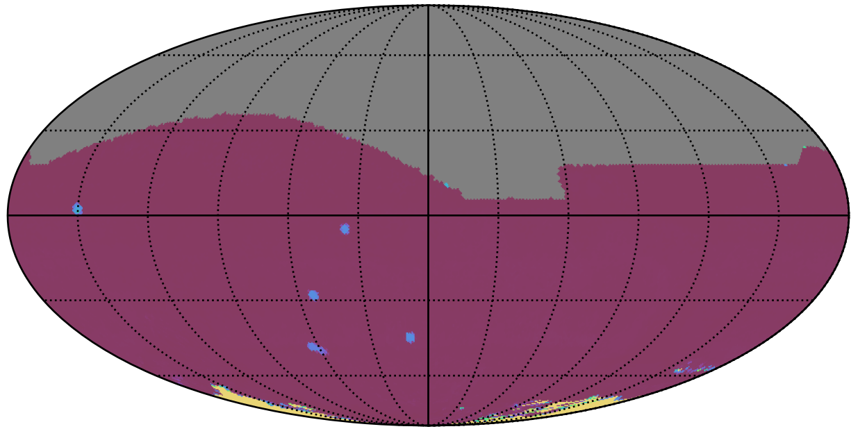
extra_ss_neo2_v3.4_10yrs All sky all bands: 75th Percentile Intranight Timespan
