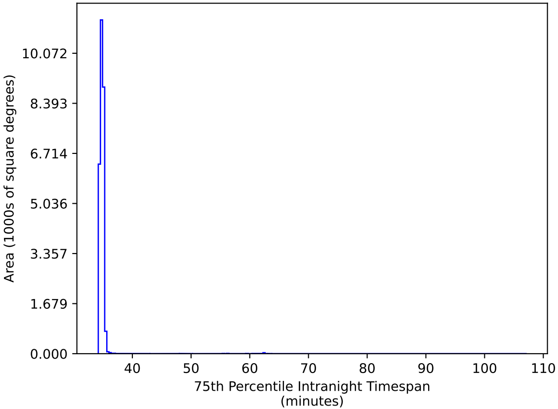
extra_ss_neo2_v3.4_10yrs All sky: 75th Percentile Intranight Timespan
