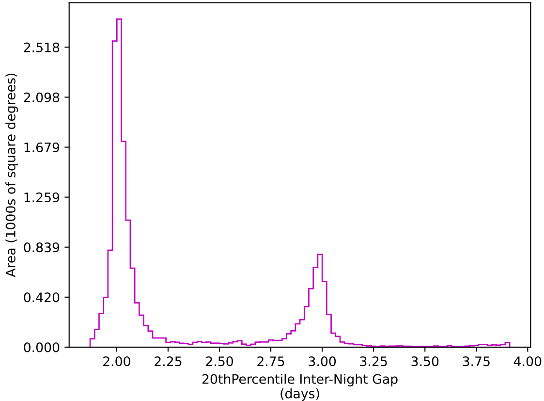
extra_ss_neo2_v3.4_10yrs WFD z band: 20thPercentile Inter-Night Gap
