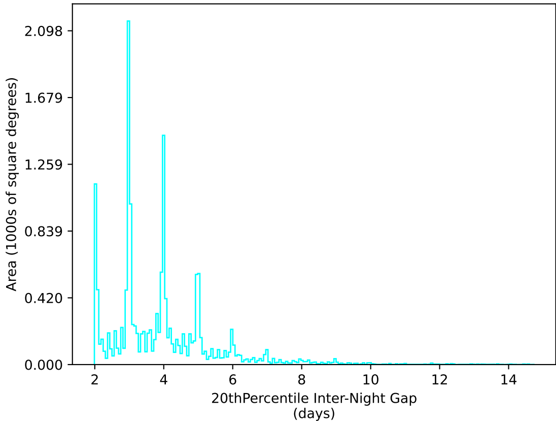
extra_ss_neo2_v3.4_10yrs WFD u band: 20thPercentile Inter-Night Gap
