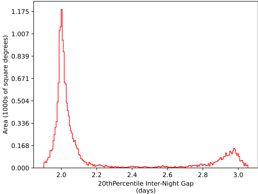
extra_ss_neo2_v3.4_10yrs WFD i band: 20thPercentile Inter-Night Gap
