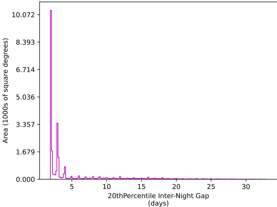
extra_ss_neo2_v3.4_10yrs All sky z band: 20thPercentile Inter-Night Gap
