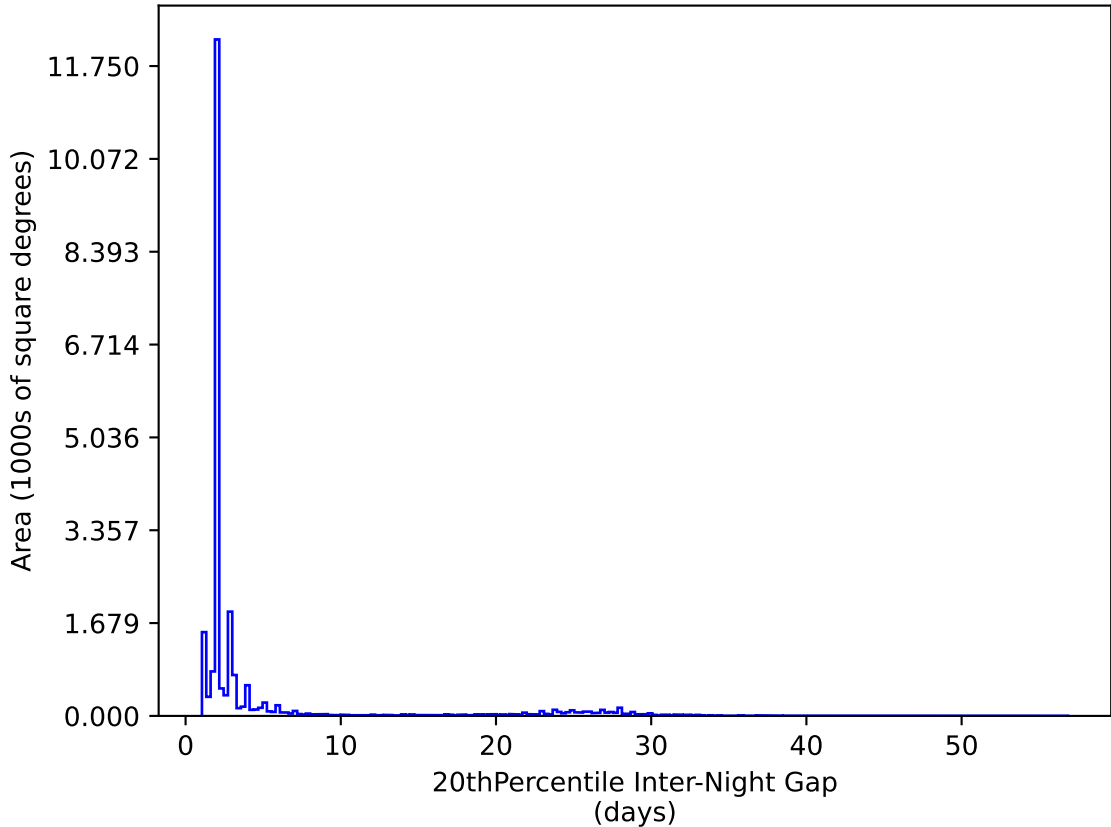
extra_ss_neo2_v3.4_10yrs All sky y band: 20thPercentile Inter-Night Gap
