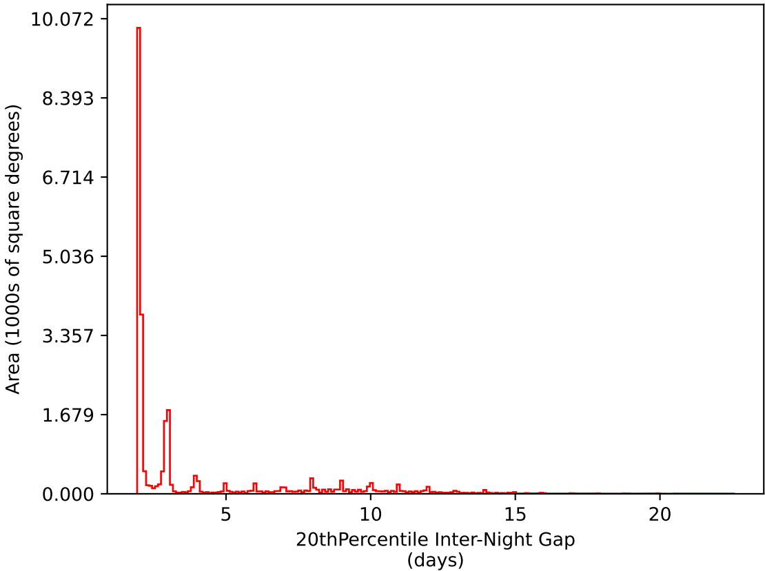
extra_ss_neo2_v3.4_10yrs All sky i band: 20thPercentile Inter-Night Gap
