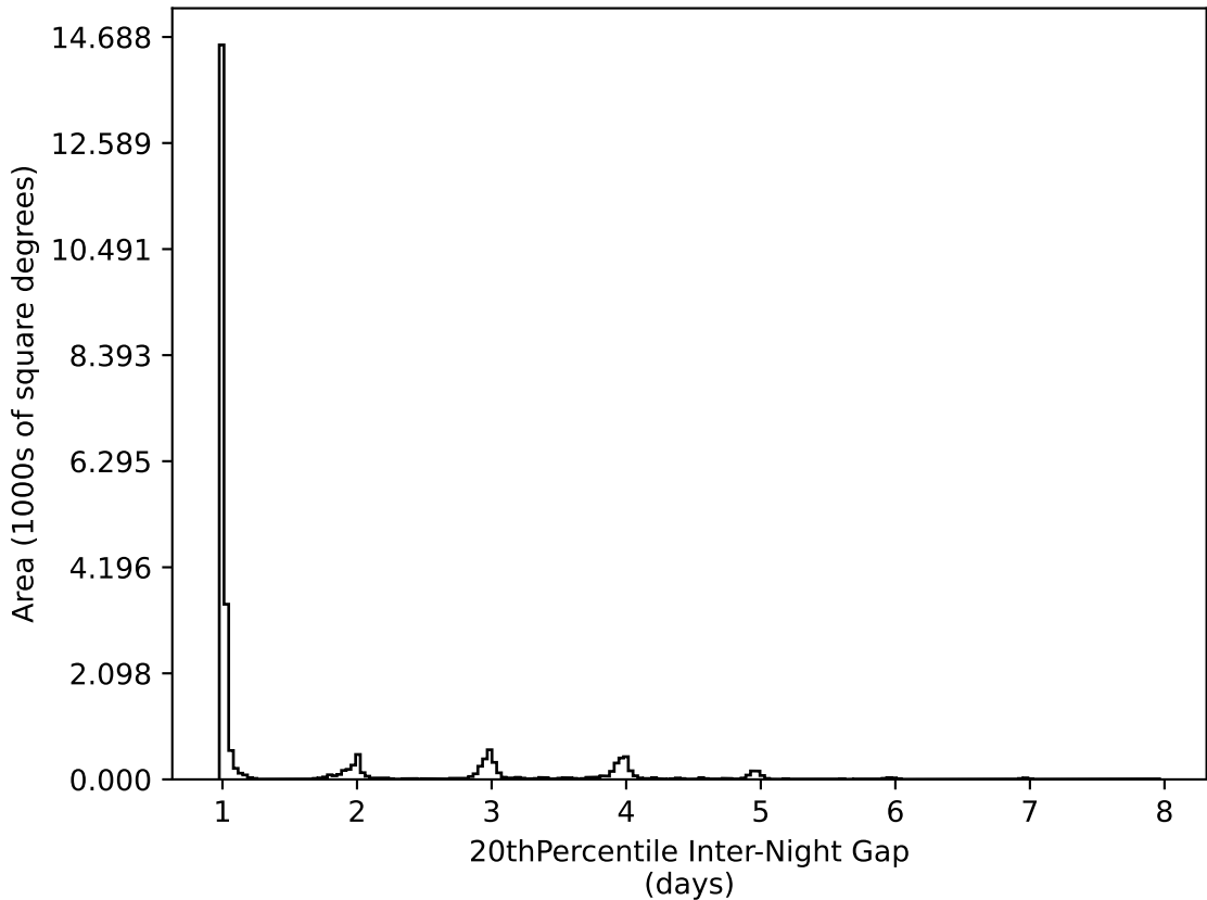
extra_ss_neo2_v3.4_10yrs All sky all bands: 20thPercentile Inter-Night Gap
