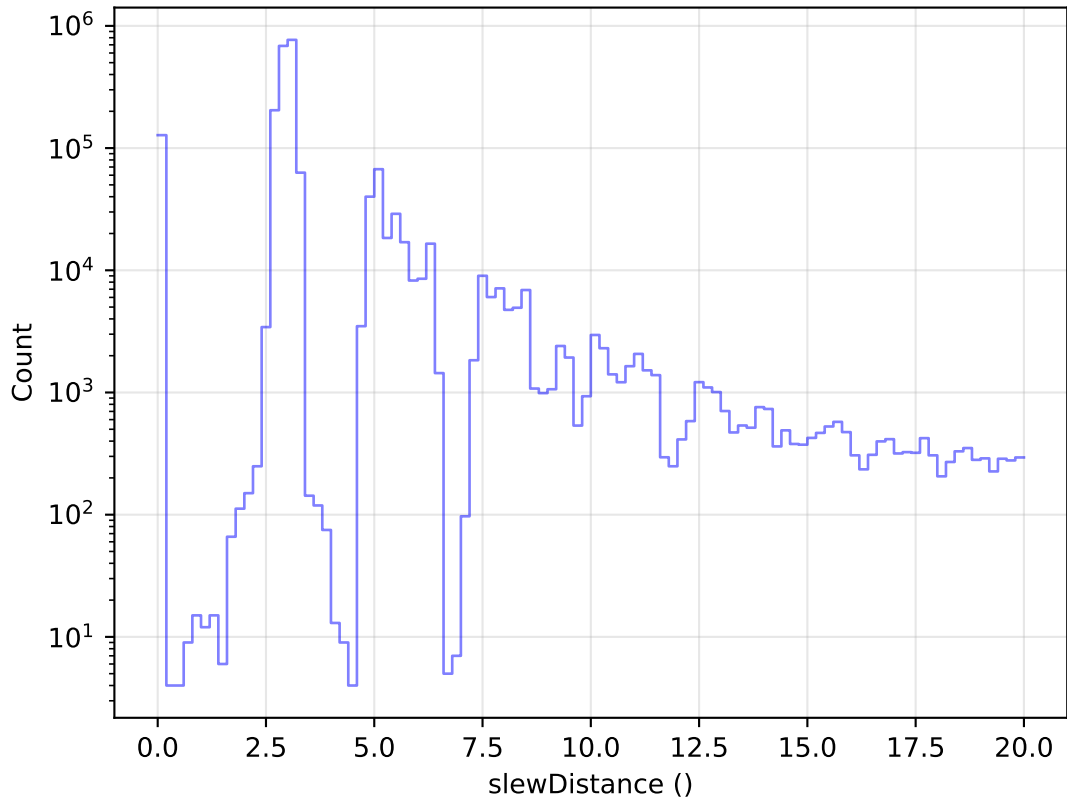
extra_ss_neo2_v3.4_10yrs All visits: Zoom Slew Distance Histogram
