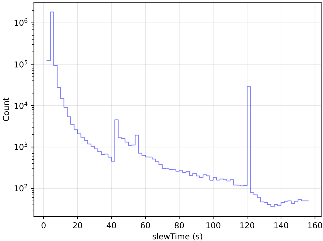
extra_ss_neo2_v3.4_10yrs All visits: Slew Time Histogram
