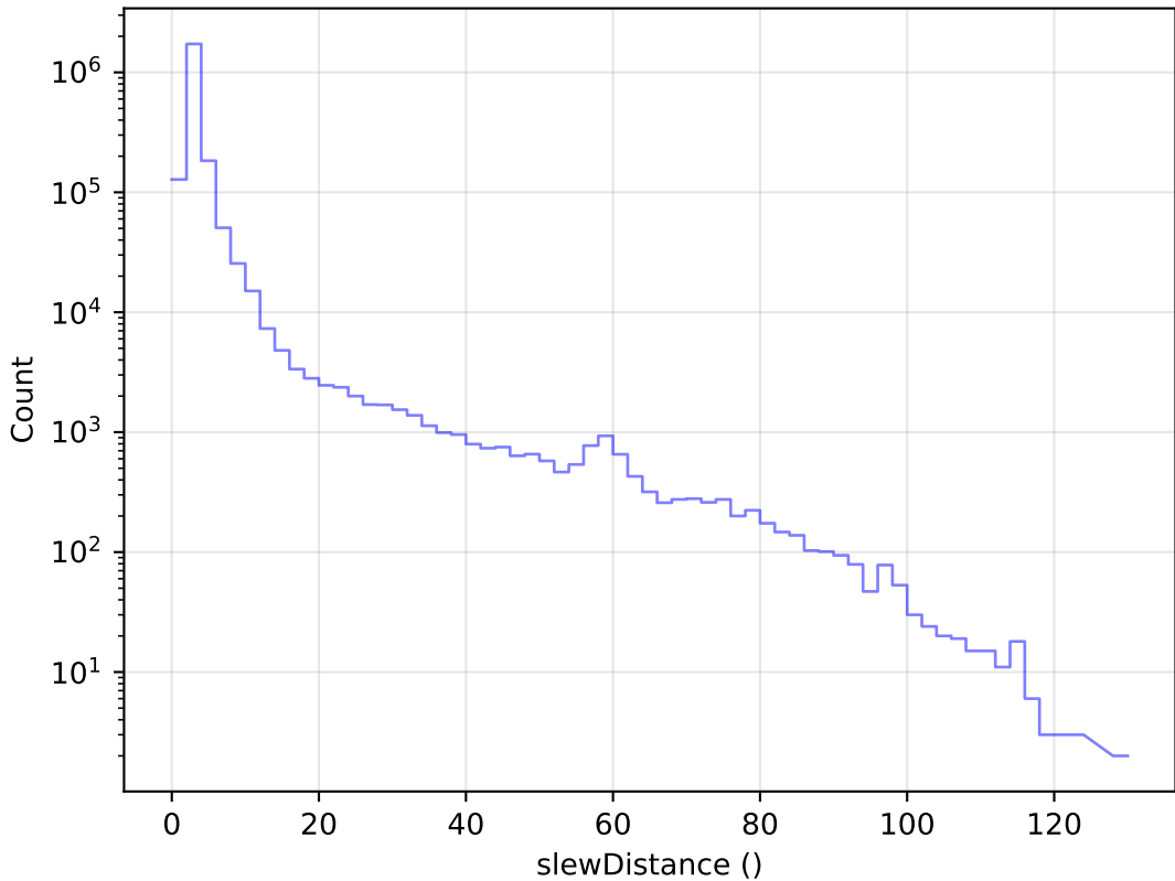
extra_ss_neo2_v3.4_10yrs All visits: Slew Distance Histogram
