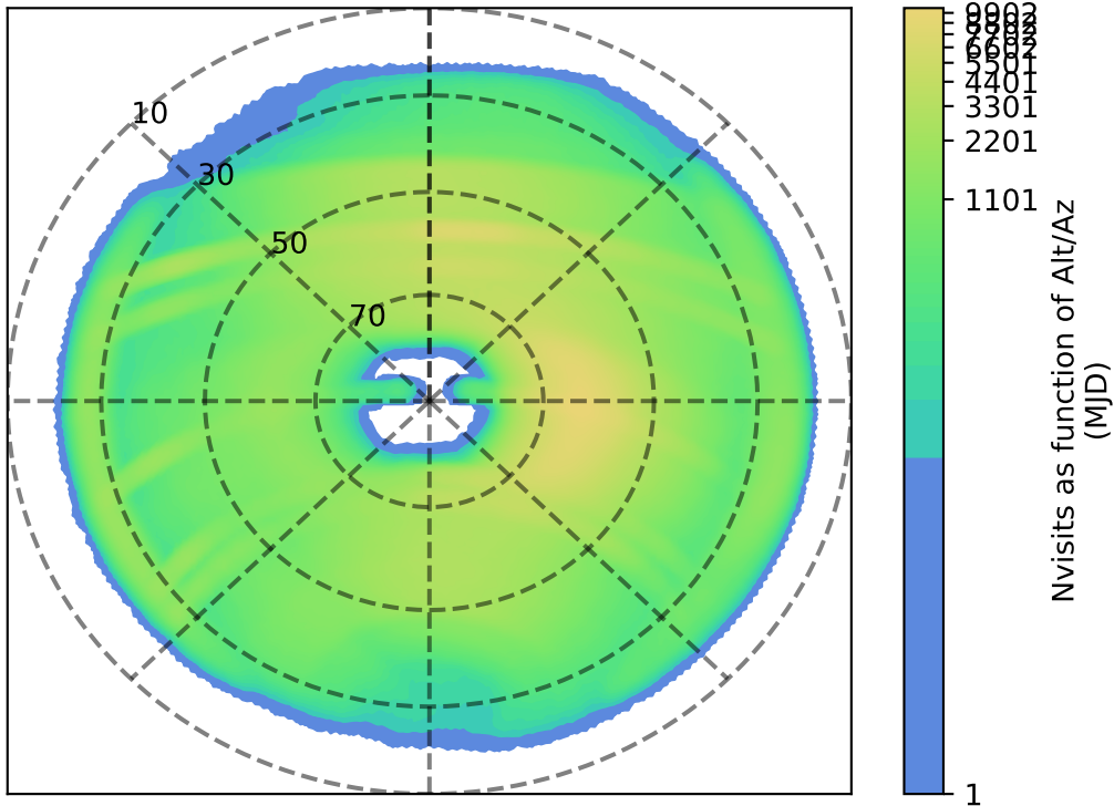
extra_ss_neo2_v3.4_10yrs : Nvisits as function of Alt/Az
