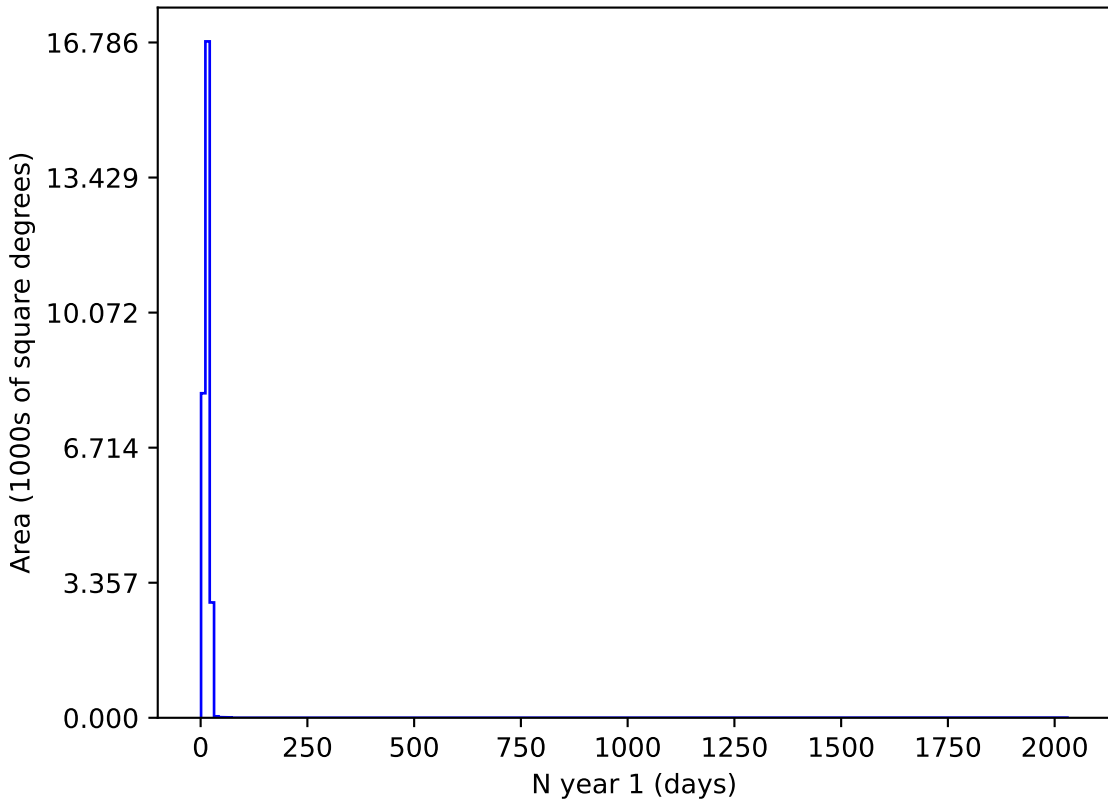
extra_ss_neo2_v3.4_10yrs z and night < 365: N year 1
