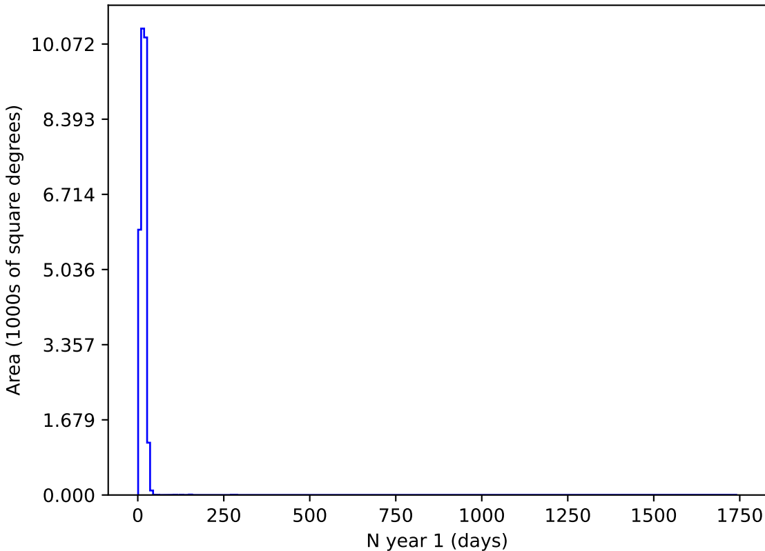
extra_ss_neo2_v3.4_10yrs r and night < 365: N year 1
