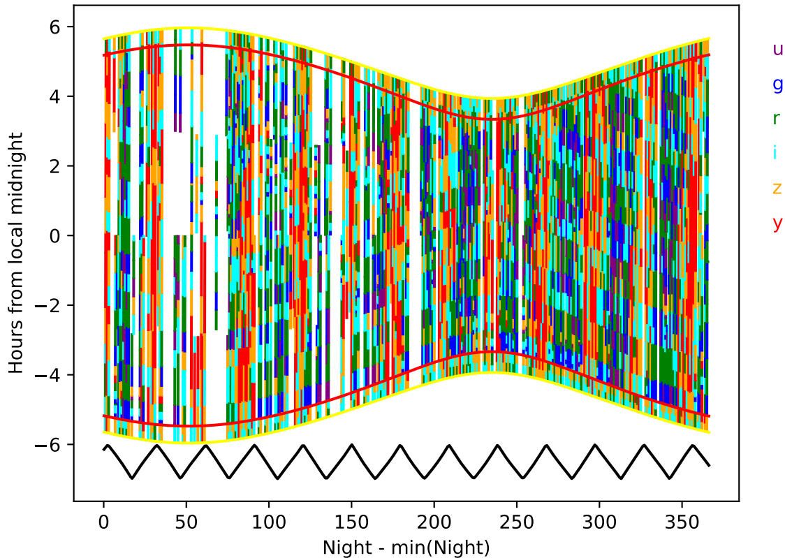
extra_ss_neo2_v3.4_10yrs year 9-10: Hourglass
