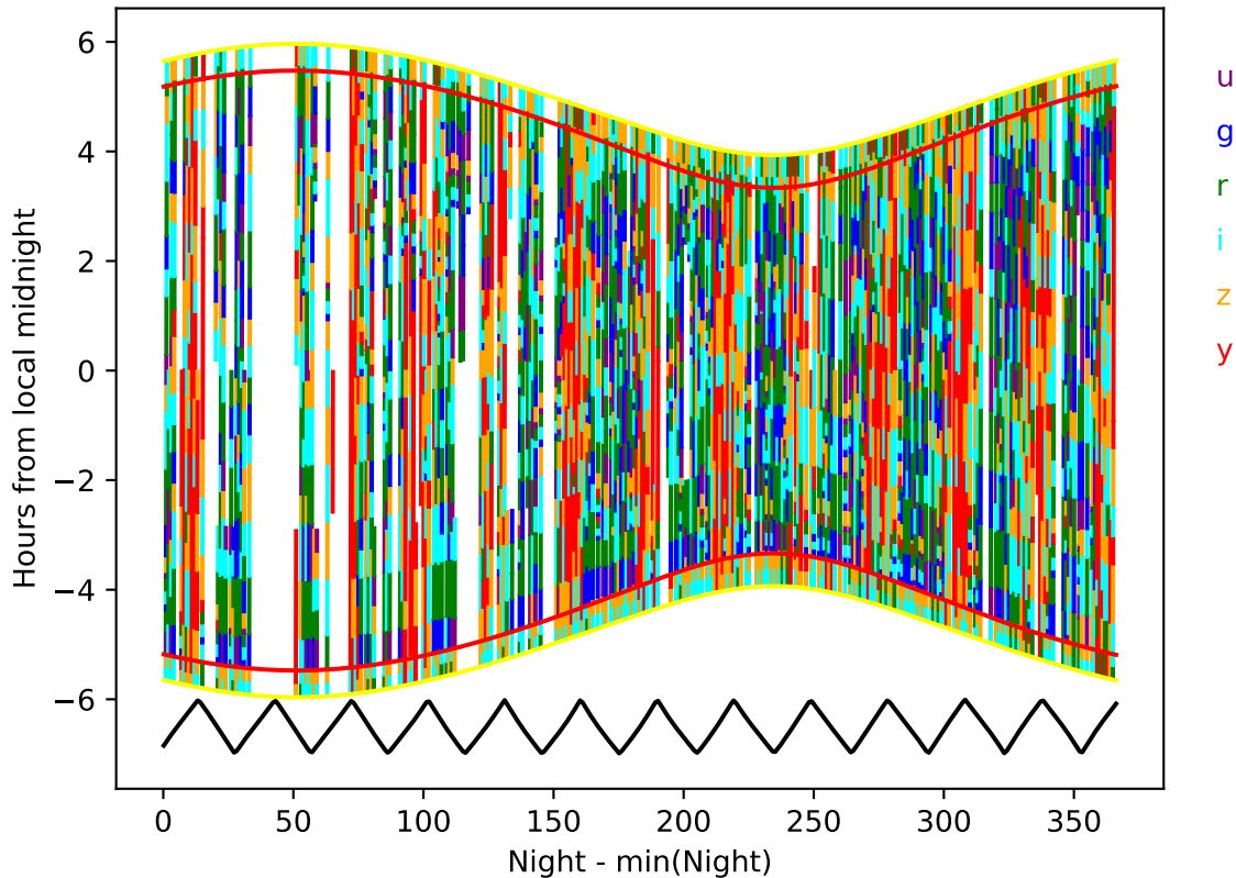
extra_ss_neo2_v3.4_10yrs year 8-9: Hourglass
