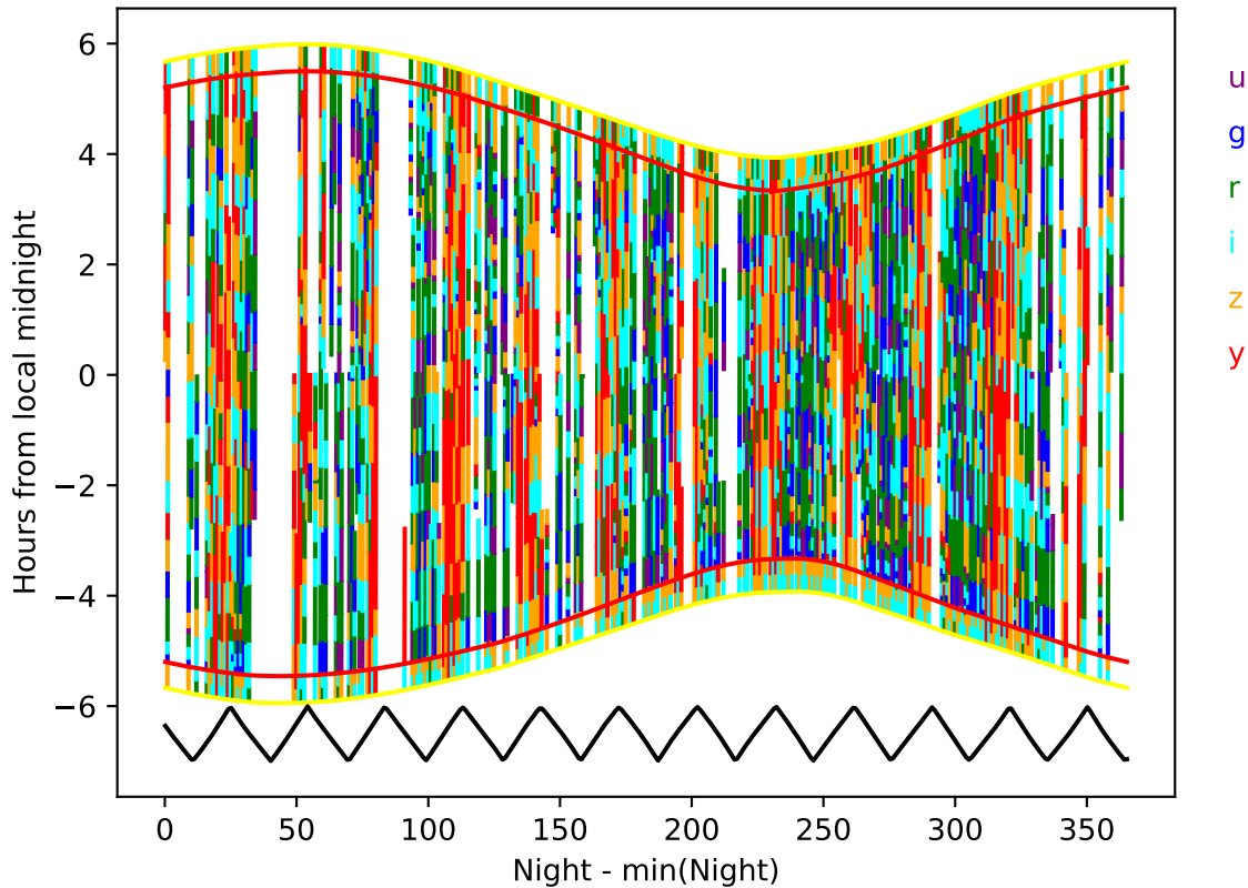
extra_ss_neo2_v3.4_10yrs year 4-5: Hourglass
