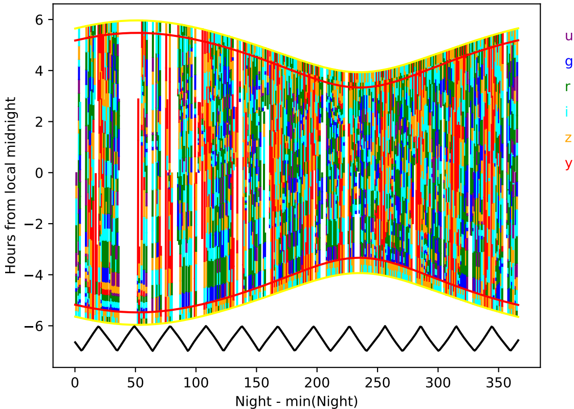
extra_ss_neo2_v3.4_10yrs year 2-3: Hourglass
