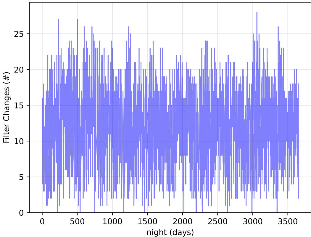
extra_ss_neo2_v3.4_10yrs : Filter Changes
