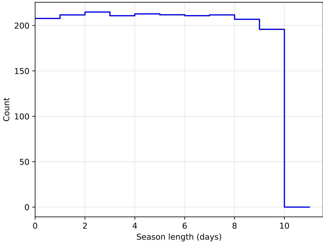
extra_ss_neo2_v3.4_10yrs DD:EDFS all bands: SeasonLength
