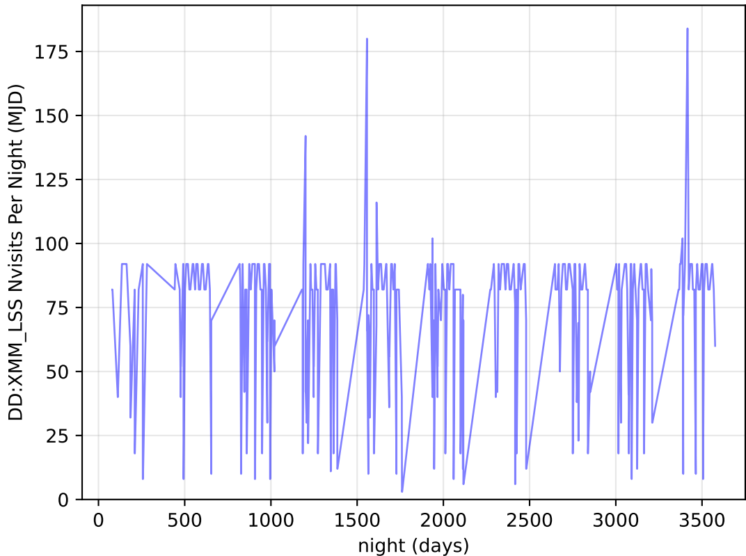
extra_ss_neo2_v3.4_10yrs all bands: DD:XMM_LSS Nvisits Per Night
