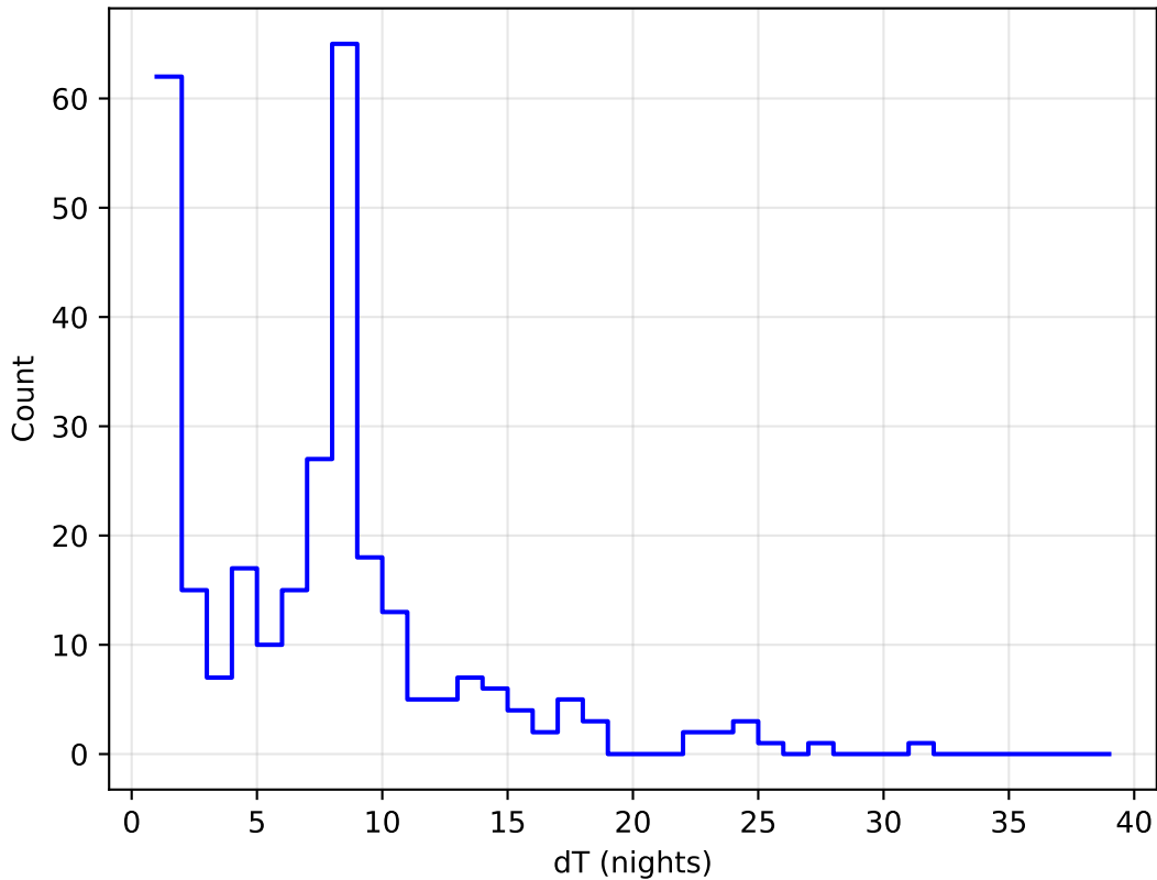
extra_ss_neo2_v3.4_10yrs all bands: DD:XMM_LSS Delta Nights Histogram
