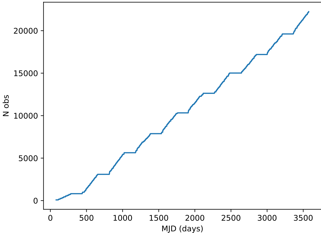
extra_ss_neo2_v3.4_10yrs all bands: DD:XMM_LSS Cumulative NVisits
