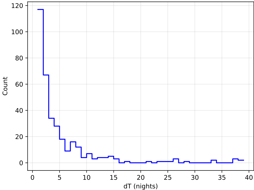
extra_ss_neo2_v3.4_10yrs all bands: DD:WFD Delta Nights Histogram
