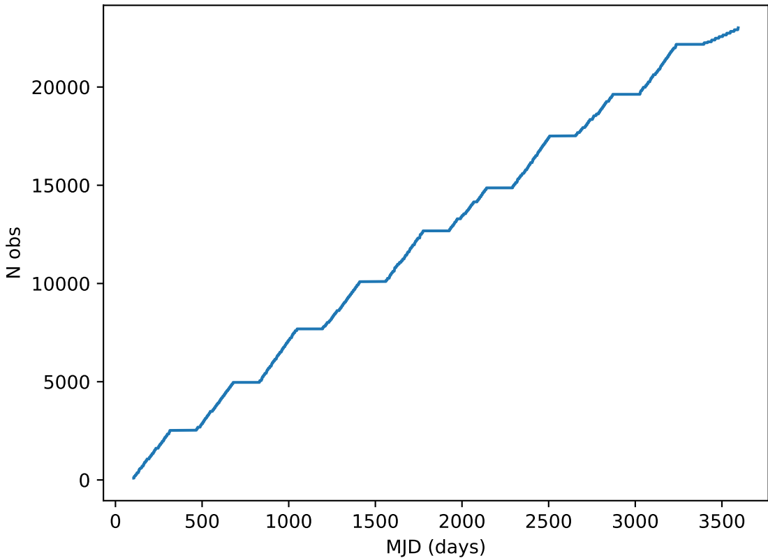
extra_ss_neo2_v3.4_10yrs all bands: DD:EDFS Cumulative NVisits
