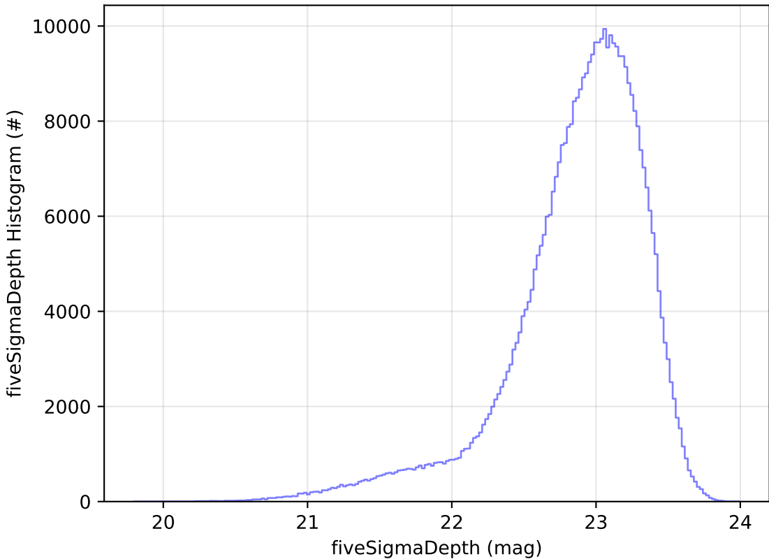
early_u_fpextra4.0_v3.4_10yrs z: fiveSigmaDepth Histogram
