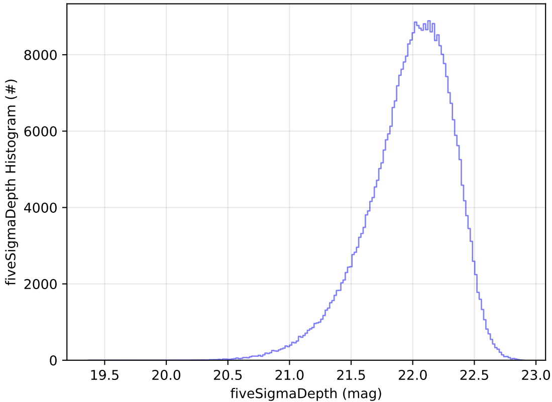
early_u_fpextra4.0_v3.4_10yrs y: fiveSigmaDepth Histogram
