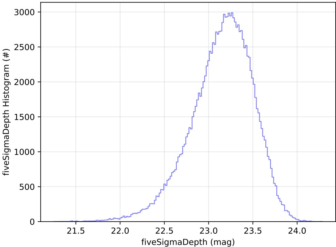
early_u_fpextra4.0_v3.4_10yrs u: fiveSigmaDepth Histogram
