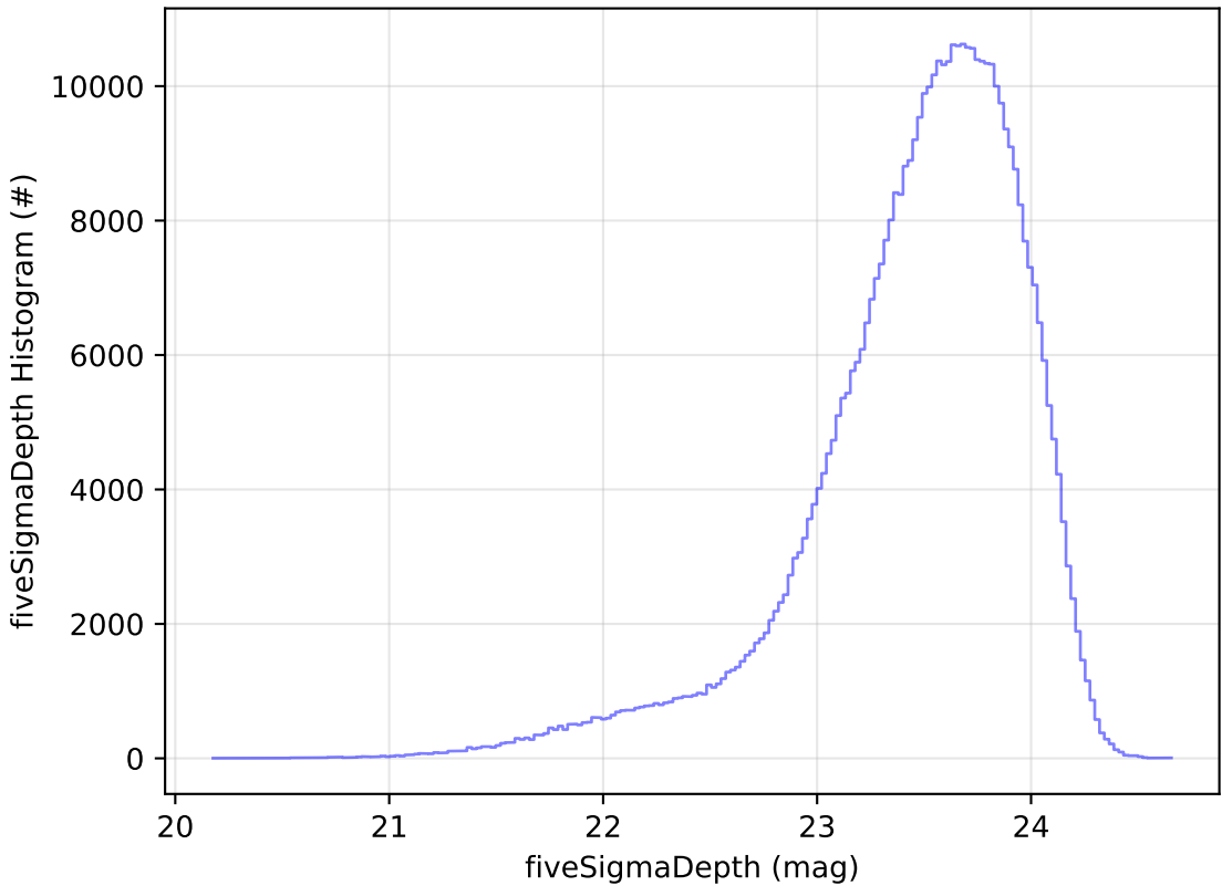
early_u_fpextra4.0_v3.4_10yrs i: fiveSigmaDepth Histogram
