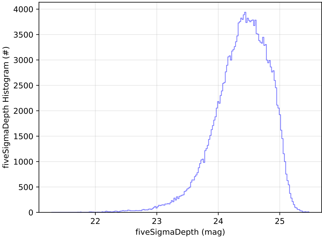
early_u_fpextra4.0_v3.4_10yrs g: fiveSigmaDepth Histogram
