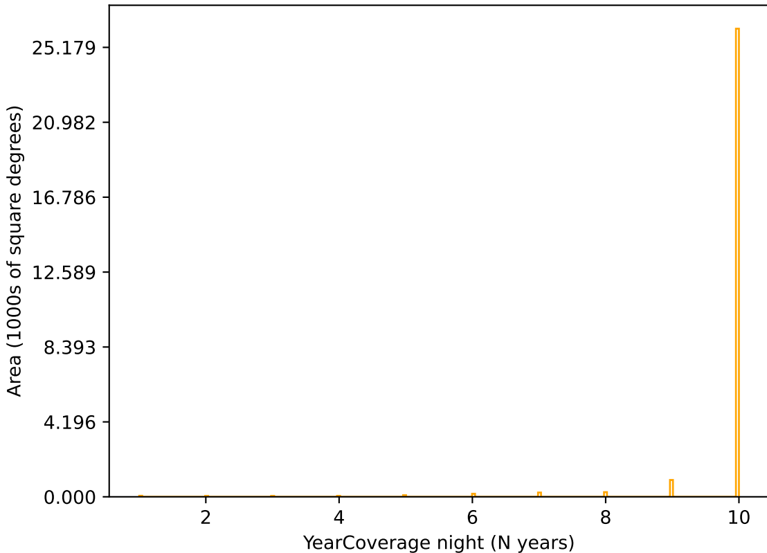
early_u_fpextra4.0_v3.4_10yrs r band: YearCoverage night
