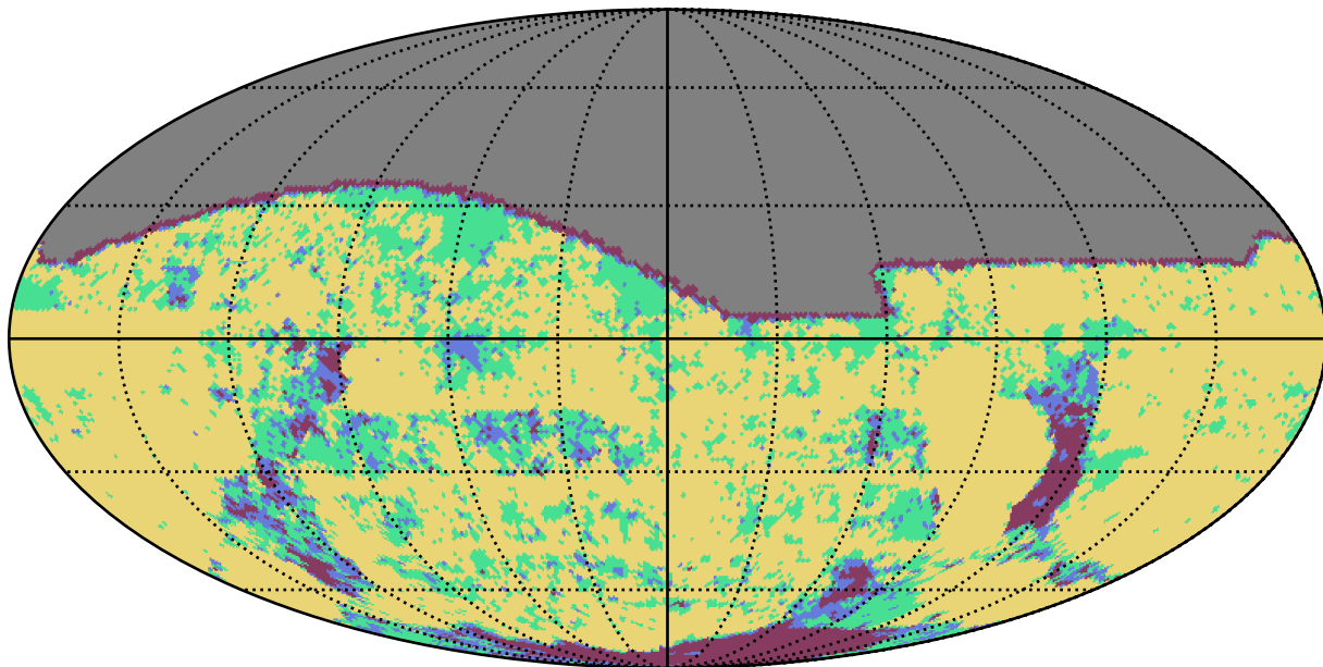
early_u_fpextra4.0_v3.4_10yrs g band: YearCoverage night
