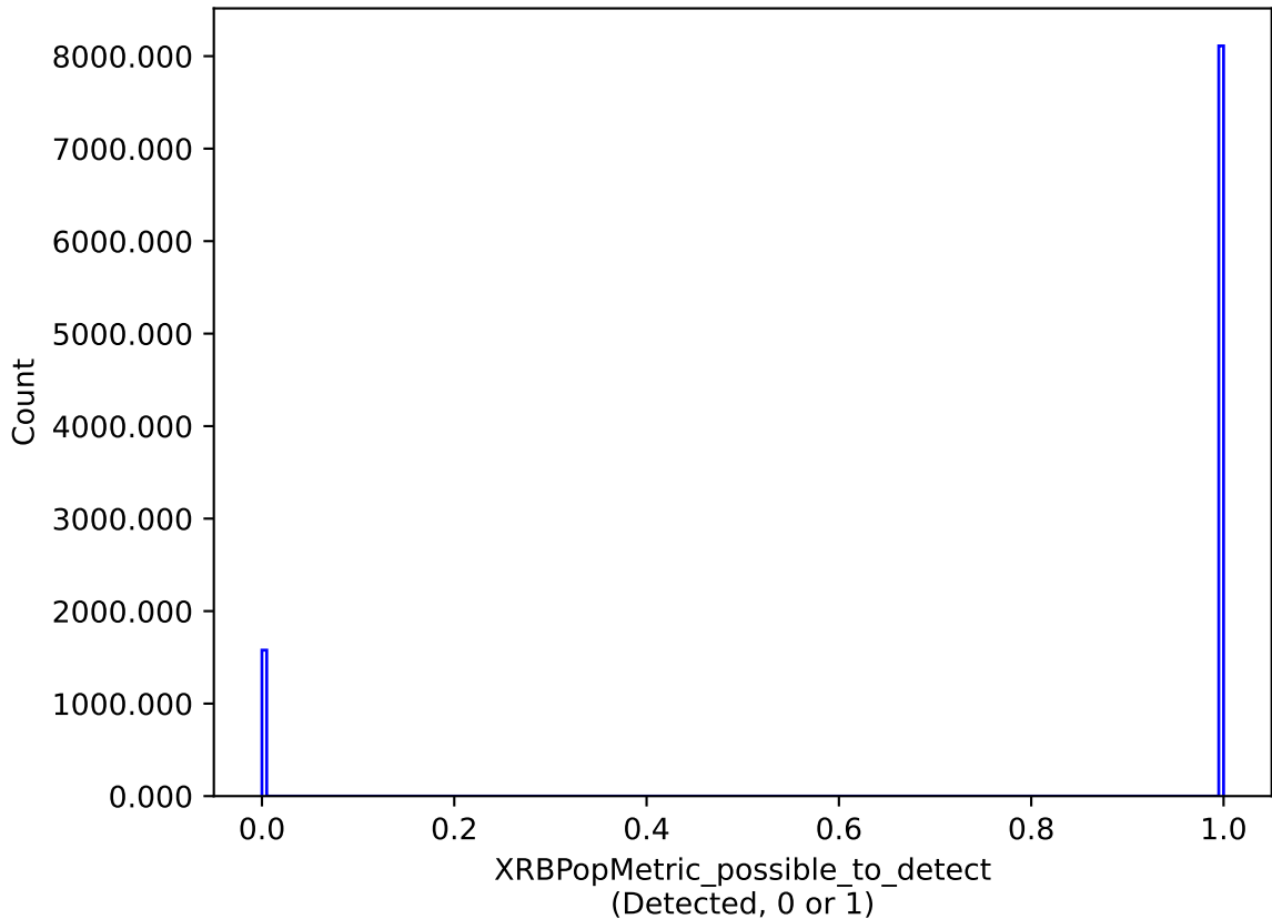
early_u_fpextra4.0_v3.4_10yrs : XRBPopMetric_possible_to_detect
