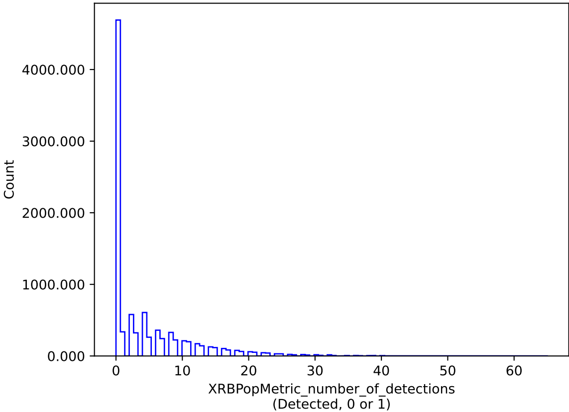
early_u_fpextra4.0_v3.4_10yrs : XRBPoMetric_number_of_detections
