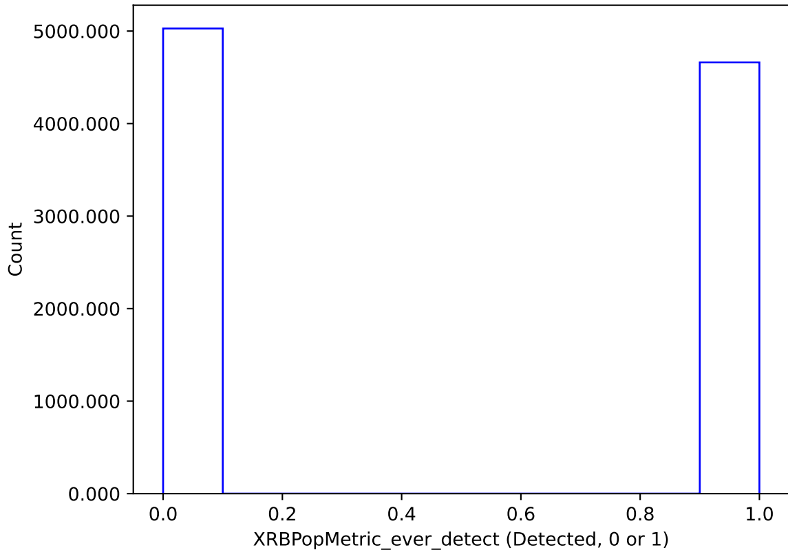
early_u_fpextra4.0_v3.4_10yrs : XRBPoMetric_ever_detect
