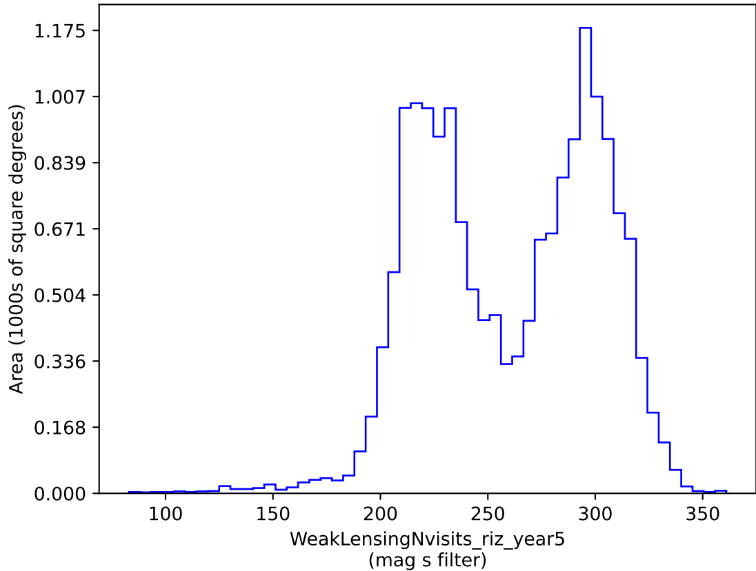
early_u_fpextra4.0_v3.4_10yrs gri band non-DD: WeakLensingNvisits_riz_year5
