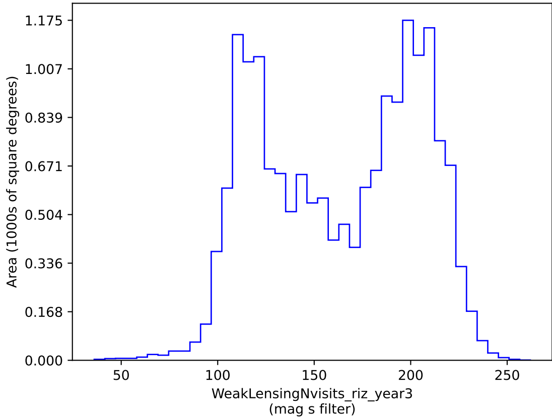
early_u_fpextra4.0_v3.4_10yrs gri band non-DD: WeakLensingNvisits_riz_year3
